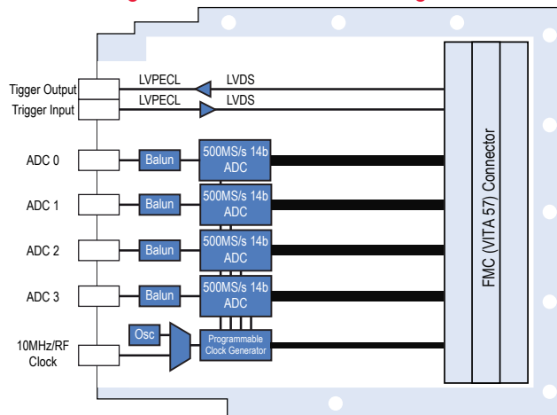
Figure 1: FMC-518 Block Diagram
